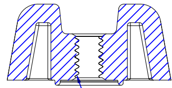
#4-40 UNC 內螺牙 SECTION A-A
