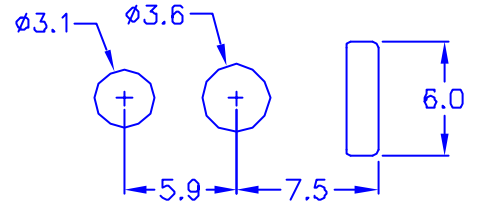
ASSEMBLY HOLE DIMENSION OF LOWER PORTION
