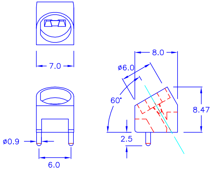
◎ HOLE IN P.C.B.:
