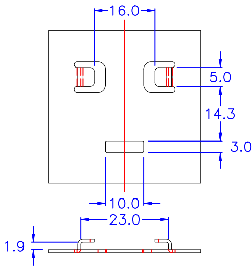
◎ CHASSIS THICKNESS: 0.8 mm
