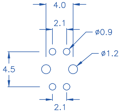
HOLE IN CHASSIS
