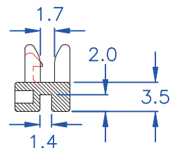
B-B SECTION
