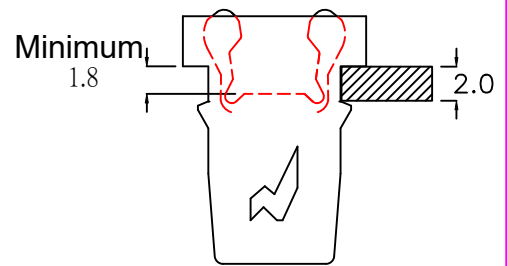
Maximum Push-Out Position
