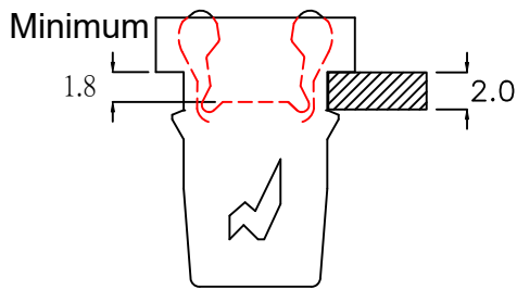
Maximum Push-IN Position
