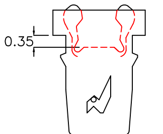
Close Position
